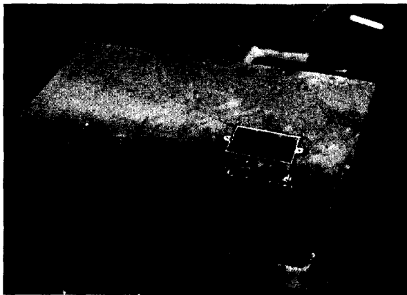
Figure 17.-Electrical outlet box mounted in sawed opening in concrete block. Box is fastened into block with 8/32 machine screws with slotted heads.
