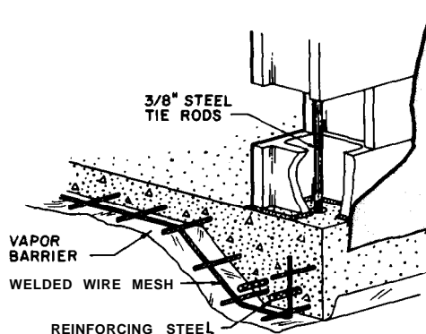
Figure 5.—Concrete slab floor on grade. Install bolts for tie-down rods.
