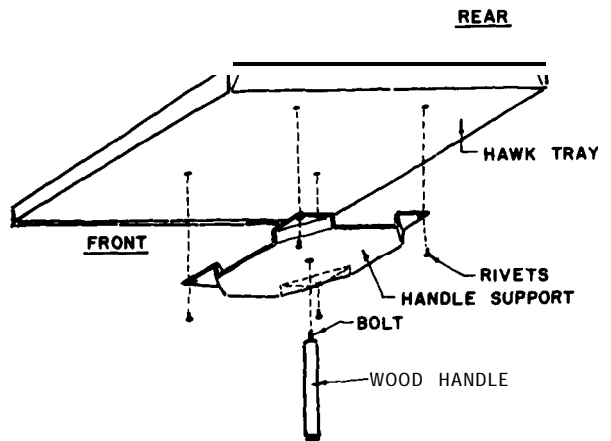
Figure Z.-Homemade hawk designed especially for surface-bonding work.
