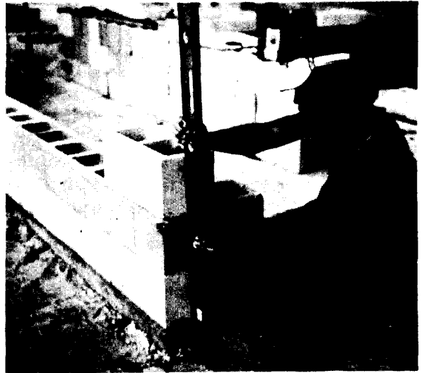
Figure 7.-Stack blocks at corners three courses high and plumb with mason's or carpenter's level.
