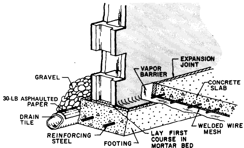
Figure 3.-Footings should be twice as wide as the wall thickness. Install drain tile adjacent to the footing to prevent buildup of water pressure against foundation. Cover open drain tile joints with 30-pound asphalted roofing felt. Backfill over tile with 12 inches of coarse gravel.
