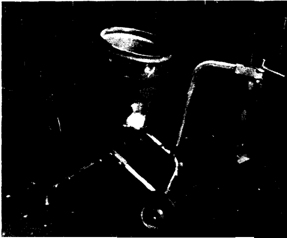
Figure 22.—Motor-driven plasterer's mixer for mixing small batches of surface bonding. The cylindrical metal container rotates against a rubber or plastic blade, creating a scraping action that does not cause the fibers to "ball up" as with other types of mixers.
