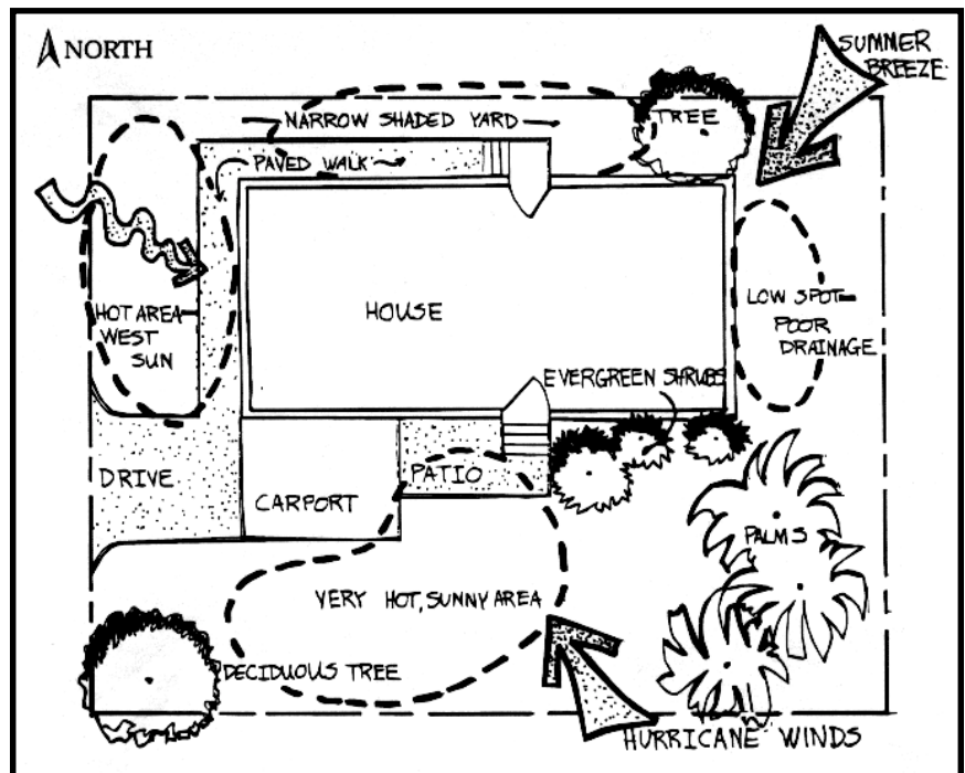
This plan drawing is for a south-facing house in a hot, humid region. Dotted lines indicate potential problem areas. The home is exposed to hurricane winds.
