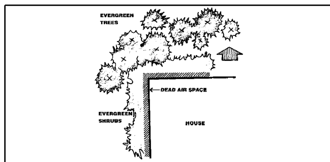
Figure 8. Windbreaks and foundation plantings will weaken the effects of cold winter winds.
