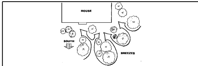
Figure 9. For passively cooled homes, trees and shrubs should be positioned to direct breezes toward windows.
