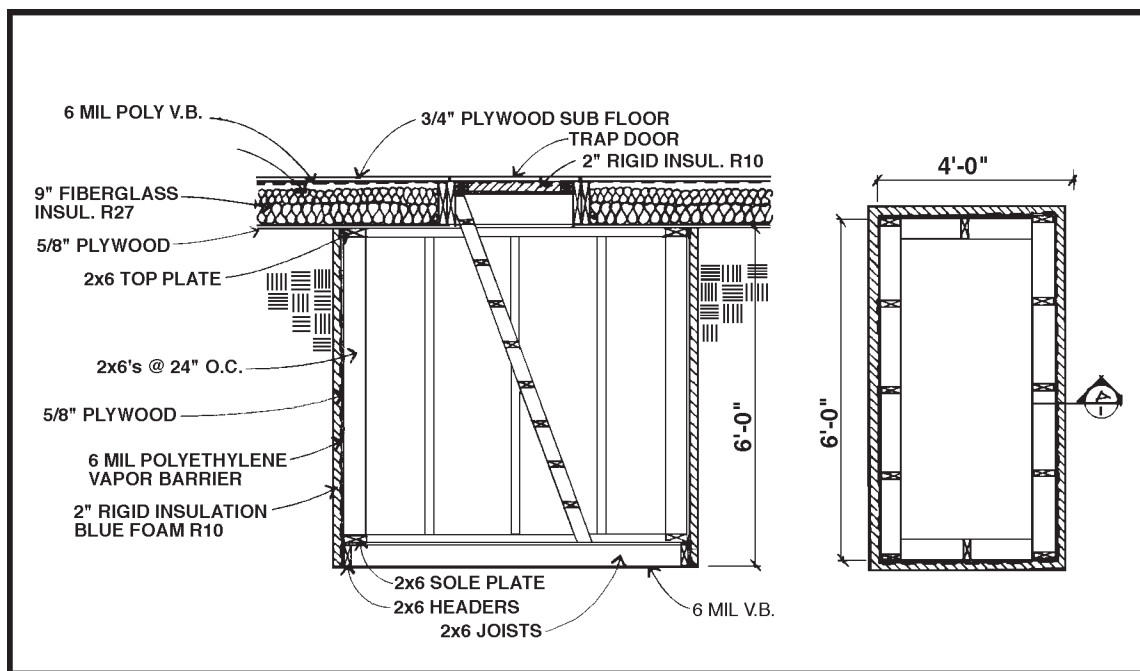
Figure 1. Example blueprint for below floor root cellar.
