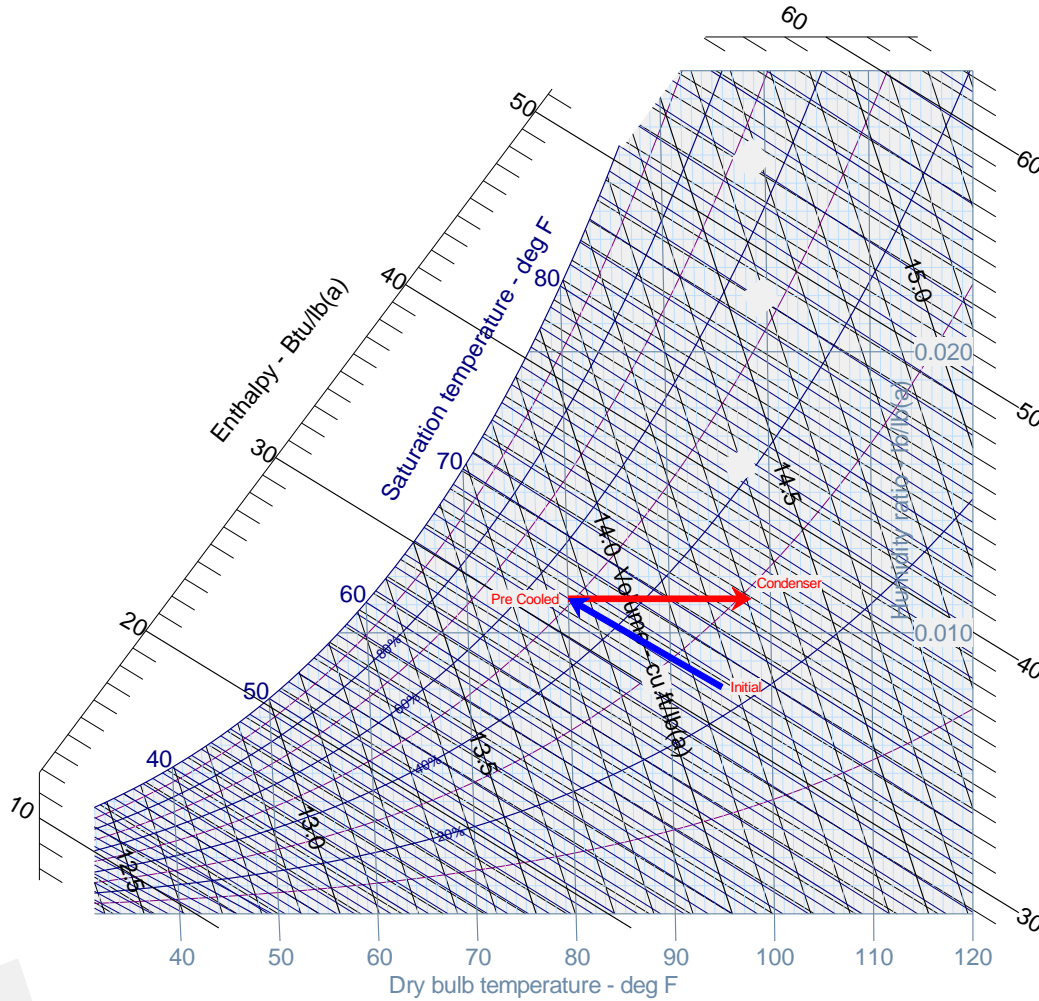
Figure 2 Psychrometric Chart
